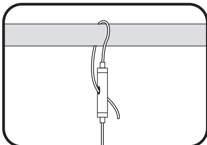
① Wrap end of cable over structural member and insert into cable gripper.
